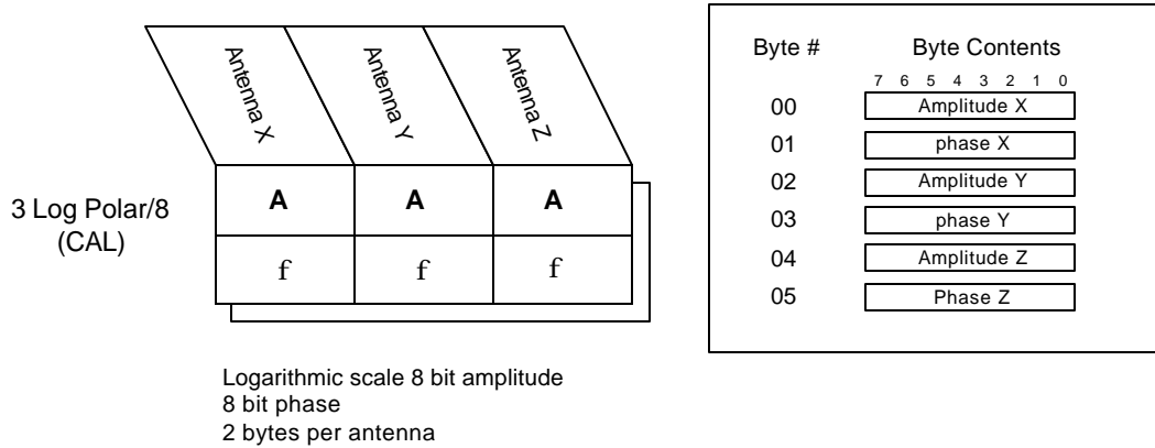
Figure 1.1-5 Calibration Data (CAL) databin
