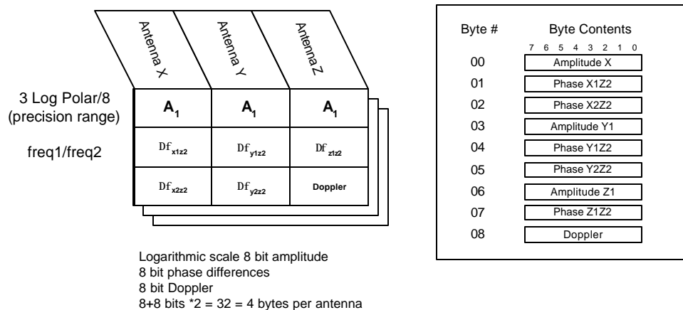
Figure 1.1-4 Precision Group Data (PRD) databin
