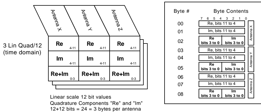
Figure 1.1-1 Linear Time Domain (LTD) databin
