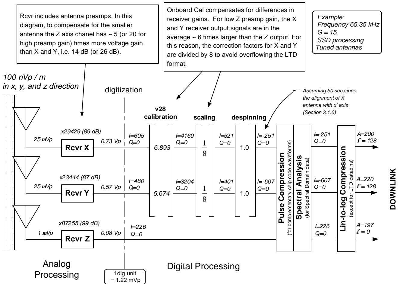
Figure 3.1-1 RPI onboard data processing.
