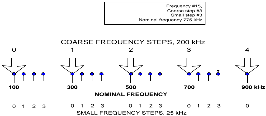
Figure 2.4-1 Example of nominal frequency calculations: linear steps, 4 multiplexed frequencies
