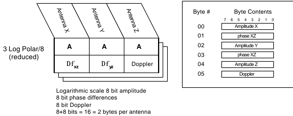
Figure 1.1-3 Spectral Maximum Data (SMD) databin
