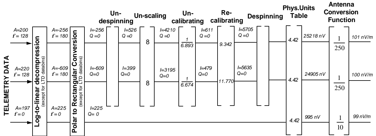
Figure 3.2-5 Conversion of amplitudes to physical units.
