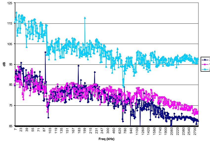
Figure 3.1-3 Voltage gain of receivers with preamplifiers for gain G = 15.
