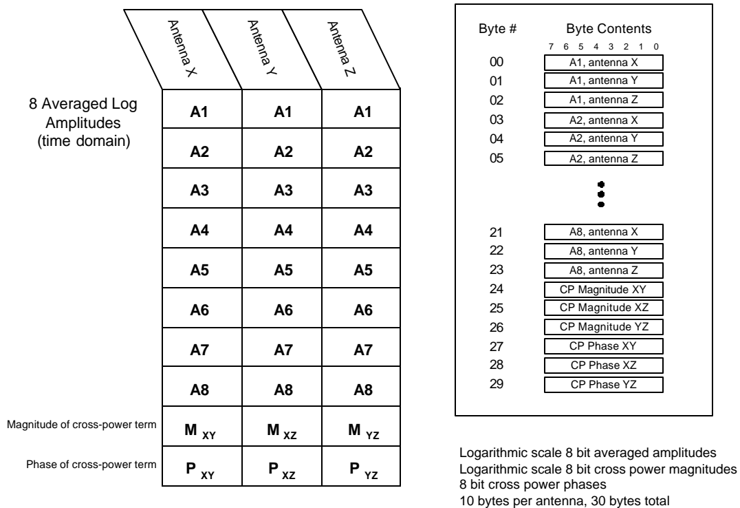
Figure 1.1-7 Thermal-noise Time-domain Data (TTD) databin
