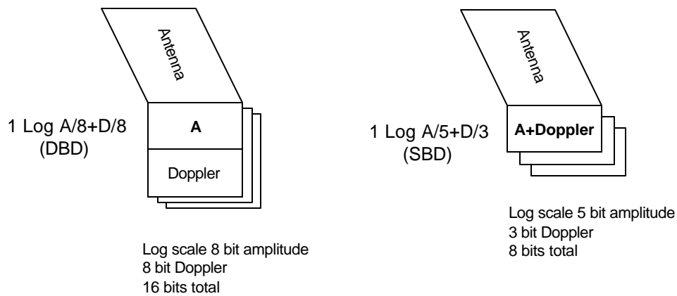
Figure 1.1-6 Double and Single Byte Data (DBD, SBD) databins
