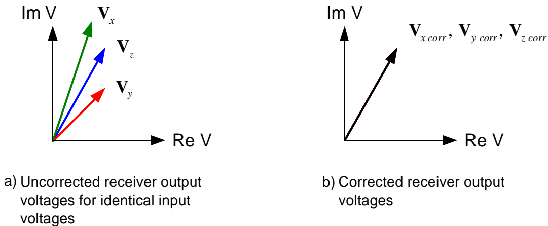
Figure 3.1-4 Desired effect of amplitude and phase corrections to X and Y output voltages.
