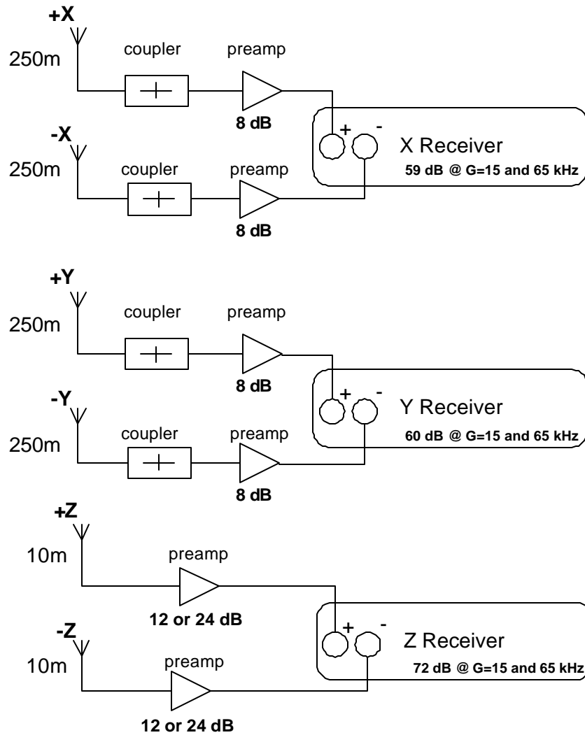
Figure 3.1-2 Three signal processing channels in RPI.
