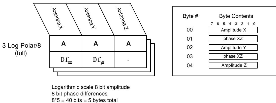
Figure 1.1-2 Spectral Science Data (SSD) databin
