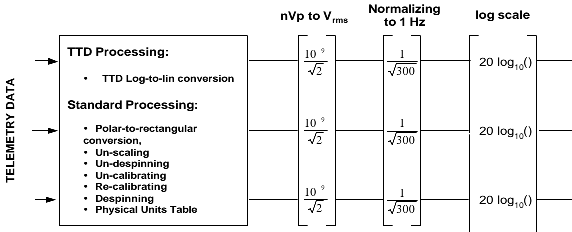
Figure 3.2-6 Physical units conversion for thermal noise data
