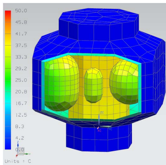
Figure B.2.7-13. Tank temperatures.
