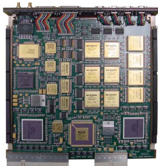
Figure B.2.7-37. The RAD750 provides high heritage for both the C&DH electronics and FSW designs.
