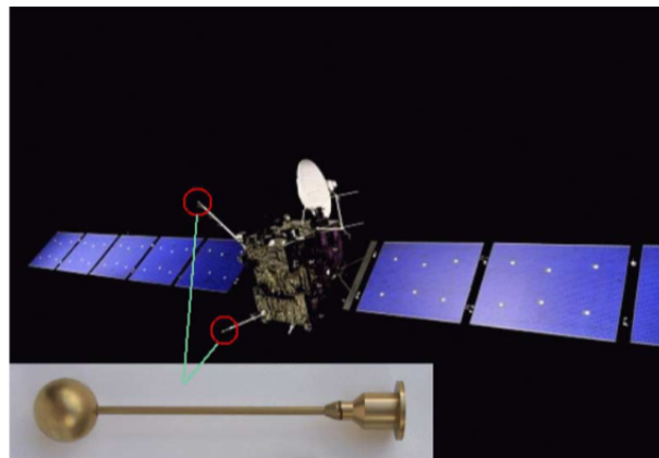
Figure B.2.5-10. The dual Langmuir Probe instrument on board Rosetta. A similar setup is considered for the Europa Orbiter.
