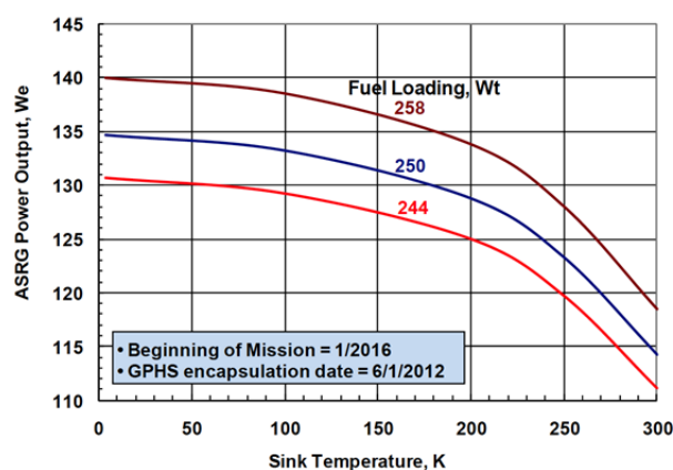
Figure B.2.7-23. ASRG output power vs. sink temperature shows that depending on the environment the output power will degrade. The ASRG power output power will depend on the view to space.
