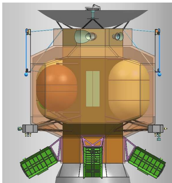
Figure B.2.7-42. Thermal enclosure.
