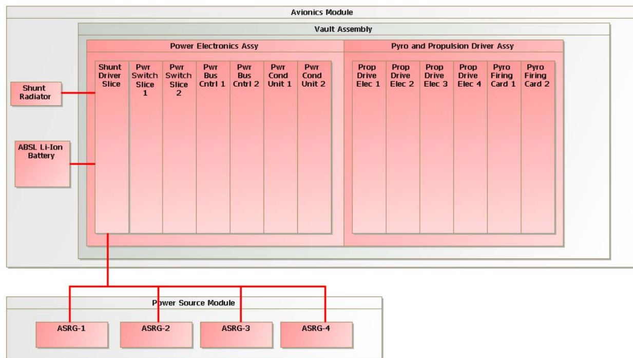
Figure B.2.7-32. Power subsystem block diagram is captured in the SysML model. The figure shows that the battery and shunt radiator are outside the vault.
