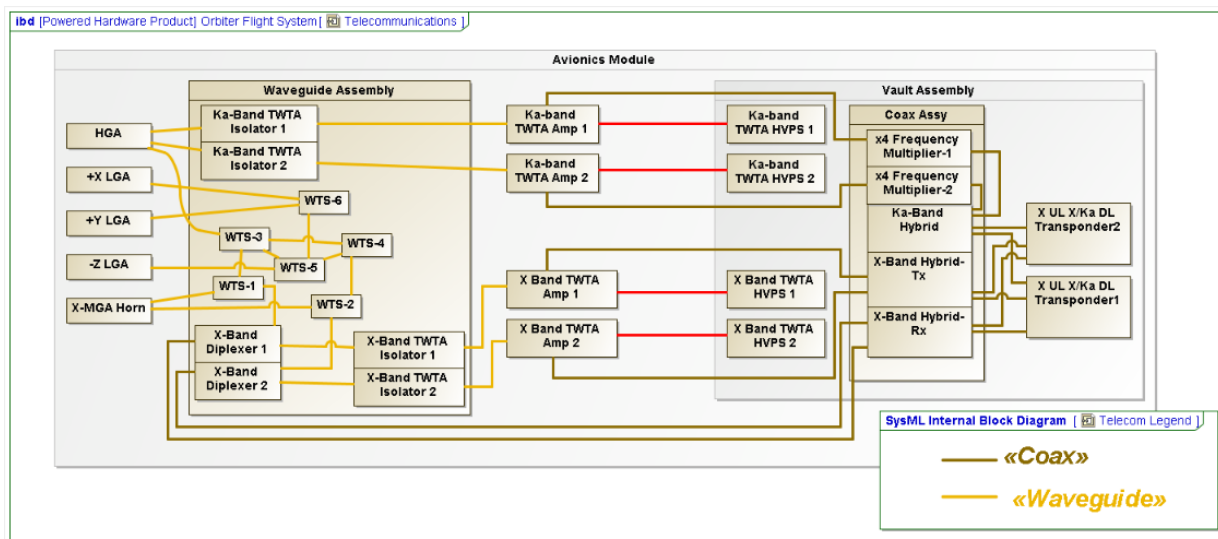
Figure B.2.7-28. The telecom subsystem provides robust fault-tolerance through a simplified architecture that minimizes potential for single-point failures.
