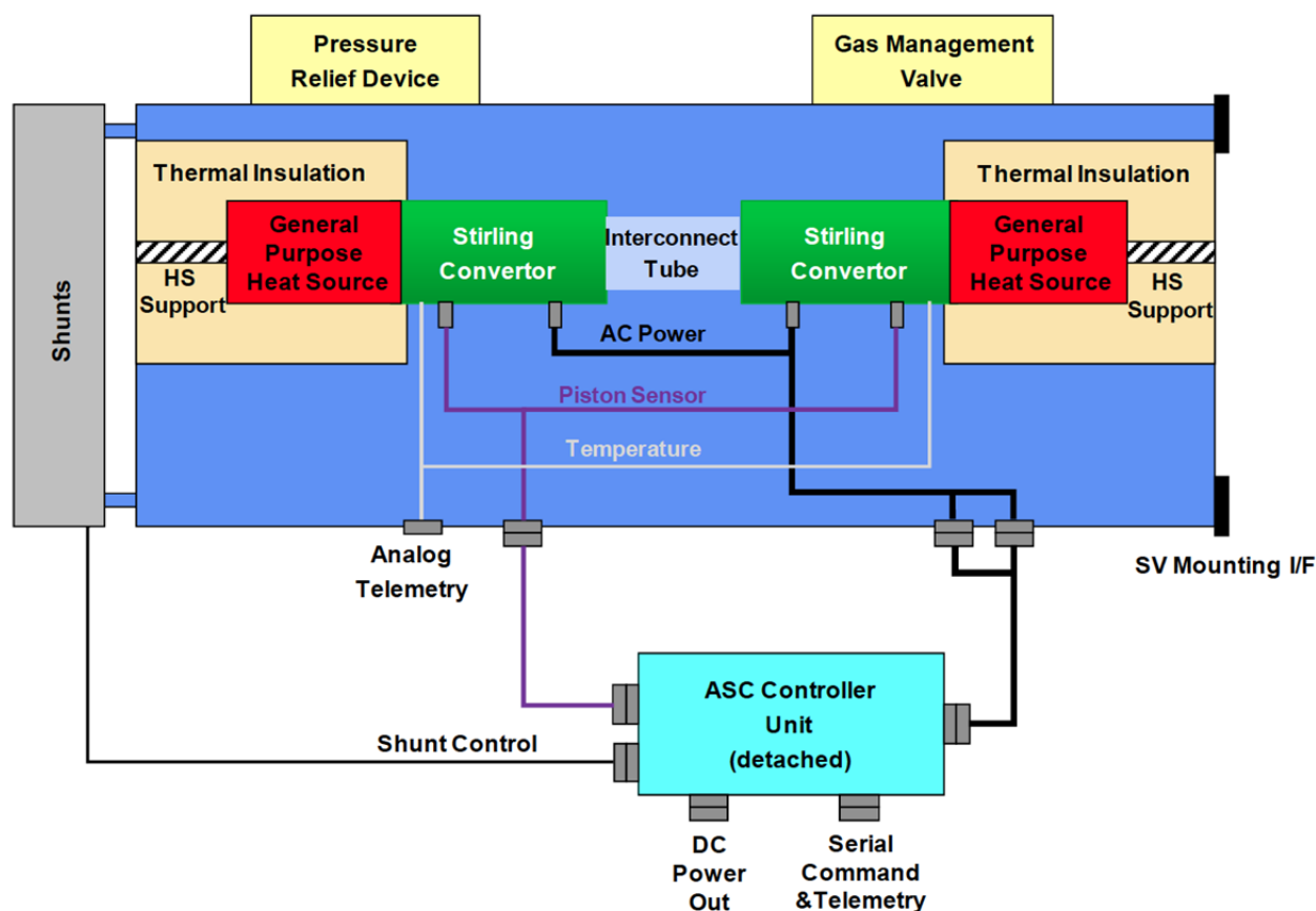
Figure B.2.7-19. The ASRG block diagram includes all functional elements that make up the ASRG, with the detached controller that provides the electrical interface with the spacecraft [HS=Heat Source].
