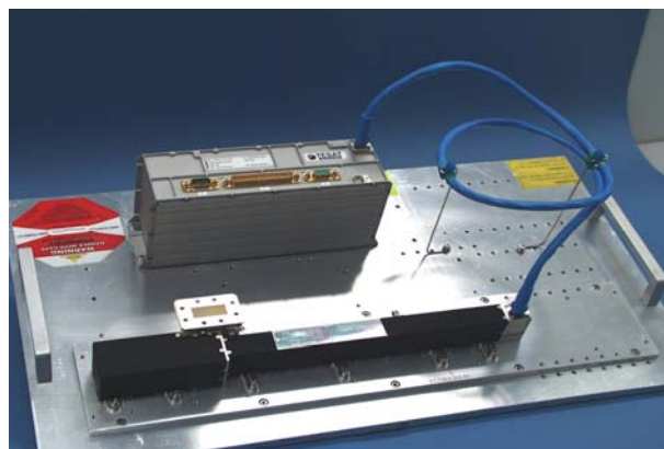
Figure B.2.7-30. Candidate X-band TWT (flown on MRO, MSL, and Dawn).
